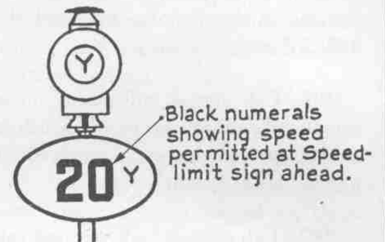
Advance Speed-limit sign
